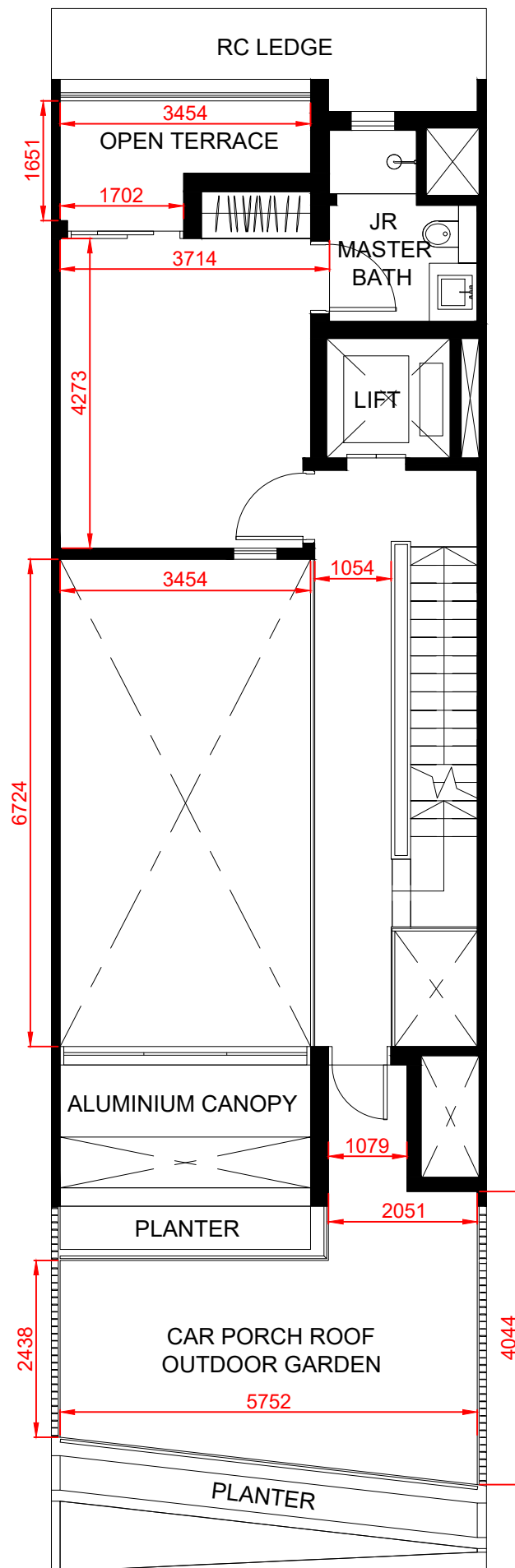
1st Storey Mezzanine
