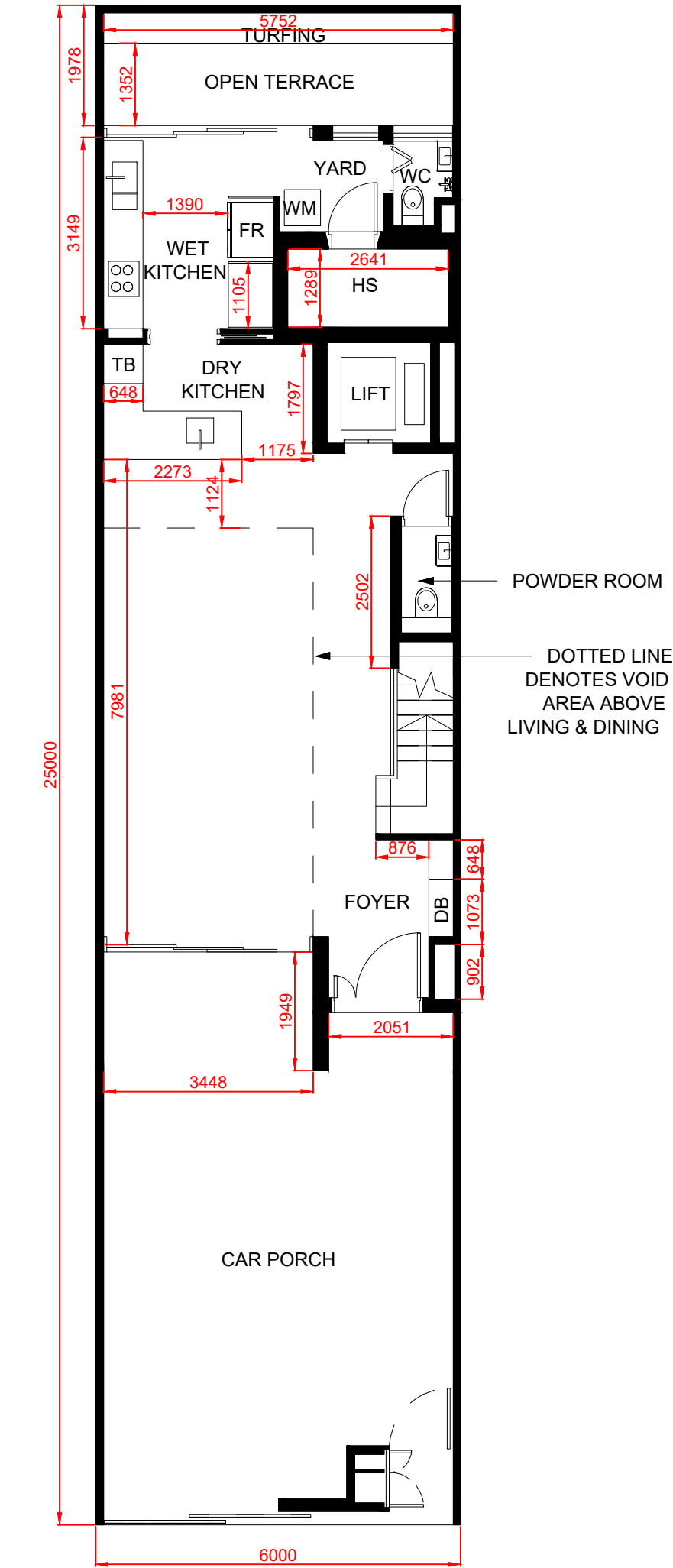
1st Storey
